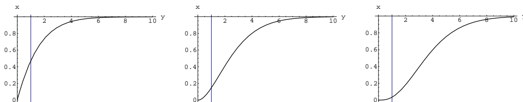
Figure 11: Left to right: x_2(y) , x_3(y) , x_4(y) .
